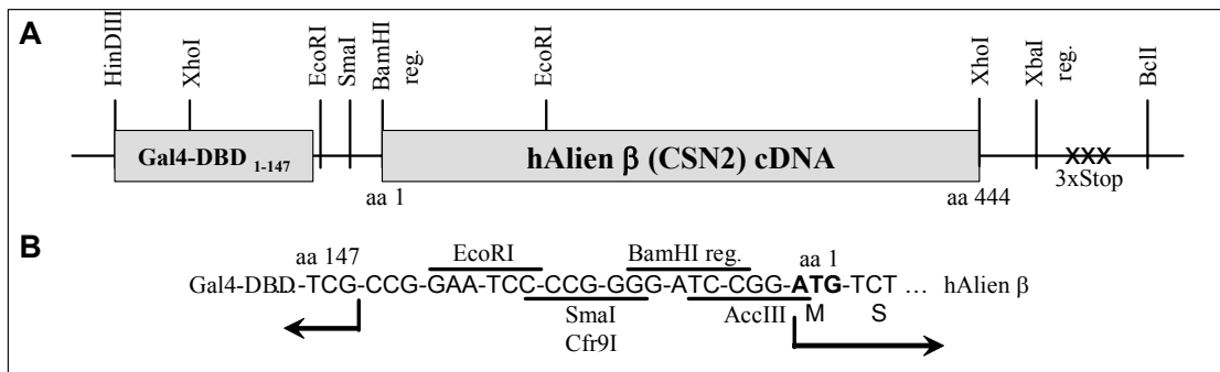
Fig. 3. Schematic view of the Gal4 fusion with hAlien β in pSG424-PUC-CSN2 (A) and the resulting sequence between the Gal4-DBD and the hAlien β cDNA, both symbolized by filled boxes (B). In frame codons are separated by hyphens. Positions of restriction sites (reg.=regenerated) and encoded amino acids (one-letter code) are labeled. xxx/3xStop indicates three stop codons in all possible frames. (C) Vector map of pSG424-PUC. The multiple cloning site and the symbolized gal4-DBD sequence coding for aa 1-147 (box; C) are shown. The Plasmid of 3.39kb contains the following elements: SV40 early promoter; Polylinker; SV40 poly A; PUC-origin of replication; Ampicillin ORF;
