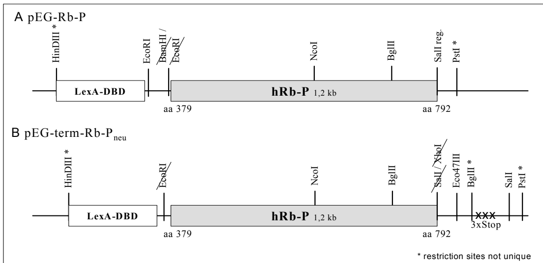
Fig. 6. Schematic view of the inserts of the plasmids pEG-Rb-P (A) and pEG-term-Rb-Pneu (B), containing the hRb pocket domain fused to the LexA-DBD (white boxes), The inserted part of hRb cDNA (grey boxes labeled hRb-P 1,2 kb) encodes the amino acid residues 379-792 of the retinoblastoma protein (pocket domain). The present restriction enzyme sites are indicated, the destroyed sites are crossed out. "xxx/3xStop" marks the existence of stop codons in all three reading frames.
