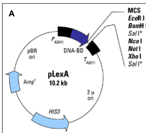
Fig. 7. Plasmide map of the pLexA-Vector (A) (originally published as pEG202, Gyuris et al., 1993) as provided by Clontech (www.clontech.com). This yeast expression plasmid codes for the LexA-DBD under the control of the alcohol-dehydrogenase promoter (PADH1). It further contains the ORF for bacterial ampicillin resistance (AmpR), the bacterial pBR-ori and the yeast 2μ-ori for replication in yeast as well as the yeast HIS3 gene for metabolic selection in suitable yeast strains. (B) shows the reading frames of the multiple cloning site of pLexA. The pLexA derivate vector pEG-term (Thormeyer) additionally contains Stop codons in all three reading frames.
