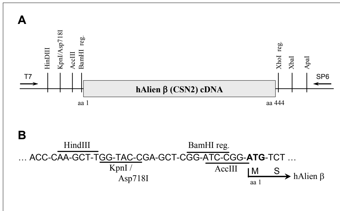
Fig. 2: Schematic representation of the hAlien \beta (CSN2) cDNA (A), inserted in pcDNA-CSN2 as well as the resulting 5'-polylinker (B). The encoded amino acids (aa) and the remaining restriction enzyme sites are indicated ("reg." means regenerated). Arrows labeled with T7 and SP6 indicate the RNA-polymerase promoters (A). In frame -codons are separated by hyphens and the first two amino acids of hAlien \beta are annotated in one letter code (B). (C). Vector map of pcDNA3, as provided by Invitrogene ( http://www.invitrogene.com ). The pcDNA3 vector used here was modified by knocking out the indicated BglII restriction site in the vector's backbone. This consisted in cutting BglII, filling in with Klenow enzyme and religation of the
