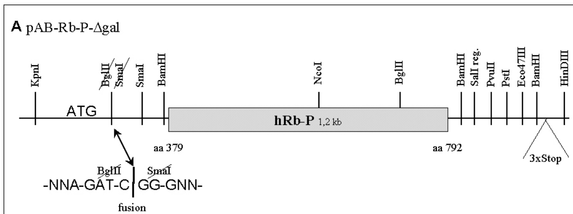
Fig 4: Schematic view of the insert of pAB-Rb-P \Delta gal, encoding the amino acid residues 379-792 (as indicated) of the human retinoblastoma protein (pocket domain of hRb; grey box). "ATG" signs the start codon, 3xStop the stop codons (in all three frames). The present restriction sites are shown, regenerated ones are labeled with "reg.", and destroyed ones are crossed out. Furthermore, the DNA sequence of the fusion is displayed (arrow) and in-frame codons are separated by hyphens
